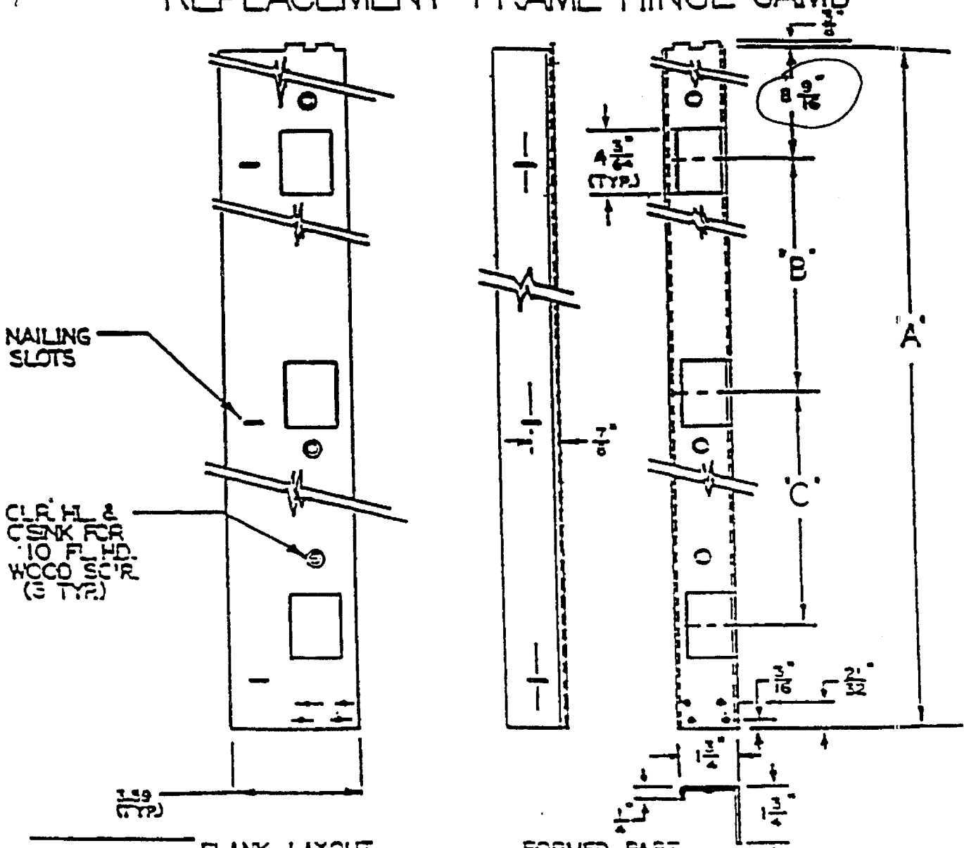
BLANK LAYOUT
